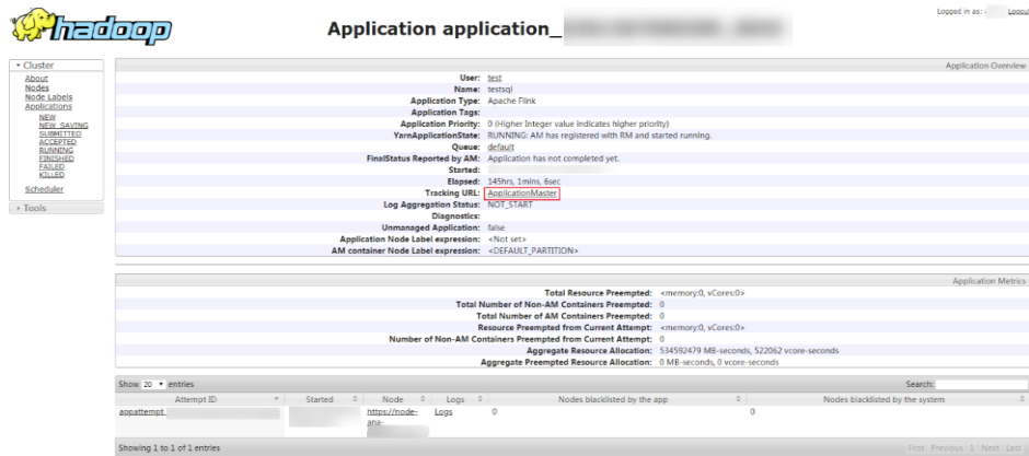
图5-4 application
