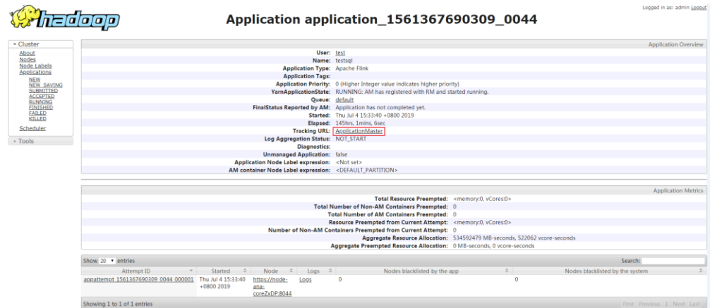
图4-7 application
