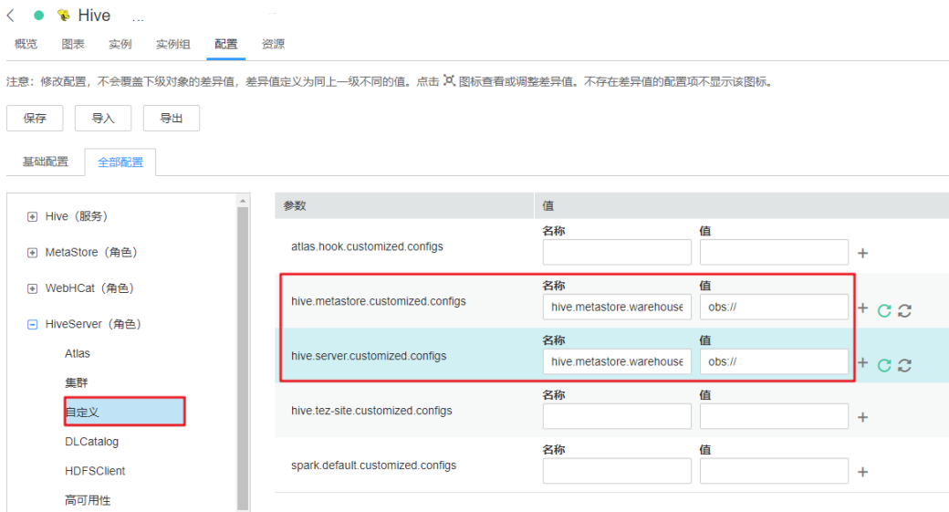
图5-12 hive.metastore.warehouse.dir 配置
