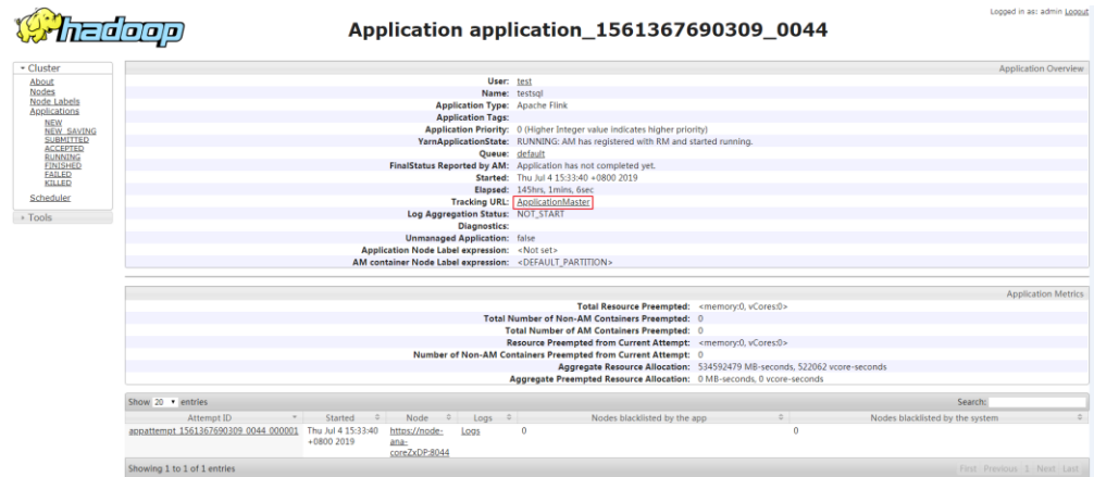
图4-11 application
